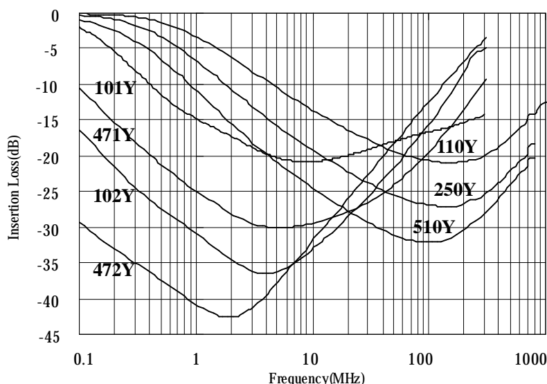
Insertion Loss vs Freq.
